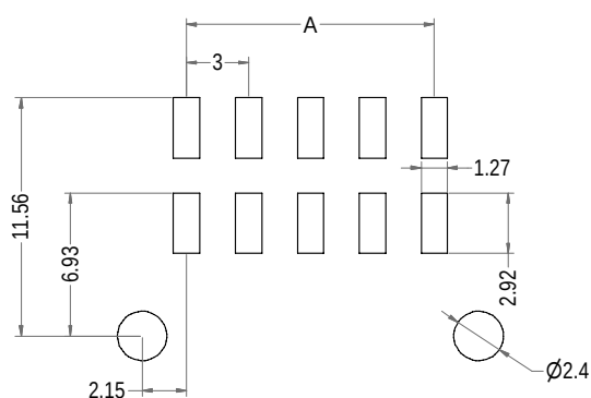
Poles Part No. Description DIM=A DIM=B 2 A3001-SRC01×2 MX3.0-2×1AWBC - 6.65 4 A3001-SRC02×2 MX3.0-2×2AWBC 3.00 9.65 6 A3001-SRC03×2 MX3.0-2×3AWBC 6.00 12.65 8 A3001-SRC04×2 MX3.0-2×4AWBC 9.00 15.65 10 A3001-SRC05×2 MX3.0-2×5AWBC 12.00 18.65 12 A3001-SRC06×2 MX3.0-2×6AWBC 15.00 21.65 14 A3001-SRC07×2 MX3.0-2×7AWBC 18.00 24.65 16 A3001-SRC08×2 MX3.0-2×8AWBC 21.00 27.65 18 A3001-SRC09×2 MX3.0-2×9AWBC 24.00 30.65 20 A3001-SRC10×2 MX3.0-2×10AWBC 27.00 33.65 22 A3001-SRC11×2 MX3.0-2×11AWBC 30.00 36.65 24 A3001-SRC12×2 MX3.0-2×12AWBC 33.00 39.65
