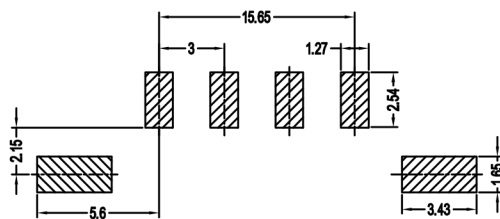
PCB LAYOUT(Tolerance:±0.05)
